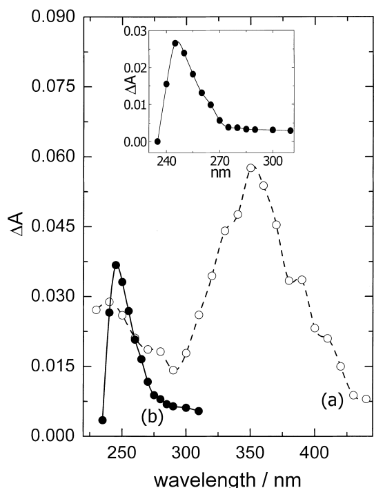
Fig. 5. Transient absorption spectra at the end of 2 \mu s pulse. (a) [CF 2 Br 2 ] = 1.4 \times 10^{-3} M, (b) [CF 2 Br 2 ] = 1.4 \times 10^{-3} M; [1,1-dimethylethanol] = 0.2 M. Inset: spectrum (b) after correction for the depletion of CF 2 Br 2 and for the absorption due to 1,1-dimethylethanol radical; dose = 108 Gy.
