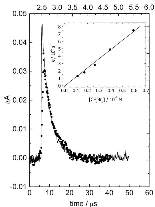
Fig. 6. Decay of e aq - at 720 nm. in blank matrix (—) (bottom x-axis) and in the presence of 2.6 \times 10^{-4} M CF 2 Br 2 (●) (top x-axis); 50 ns pulse; dose = 12 Gy. Inset: Dependence of observed rate constant on CF 2 Br 2 concentration.
