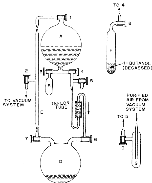
Fig. 2. Apparatus for the preparation and manipulation of aqueous solutions of \text{CF}_2\text{Br}_2 for pulse radiolysis (schematic). A: Reservoir for the preparation and storage of feed solution, total capacity = 0.6 L.; B: Ampoule to store the measured amount of \text{CF}_2\text{Br}_2 before mixing; C: Flow cell for pulse radiolysis, made from Suprasil tube of 10 mm \times 10 mm internal cross section, D: Receiver; 1–9: Grease free high vacuum stopcocks.
