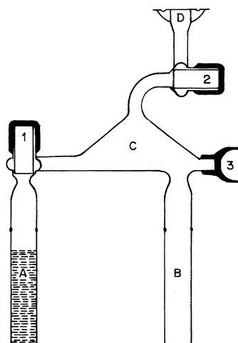
Fig. 1. Apparatus for determining the Henry's law constant ( K_h ) (schematic). A and B: Far UV Grade spectrophotometric cuvettes of 10 mm path length, A for liquid and B for gas; C: equilibration chamber; 1, 2: Grease free high vacuum stopcocks; 3: sampling port with viton/silicone rubber septum for gas chromatographic analysis; D: O-ring connector.
