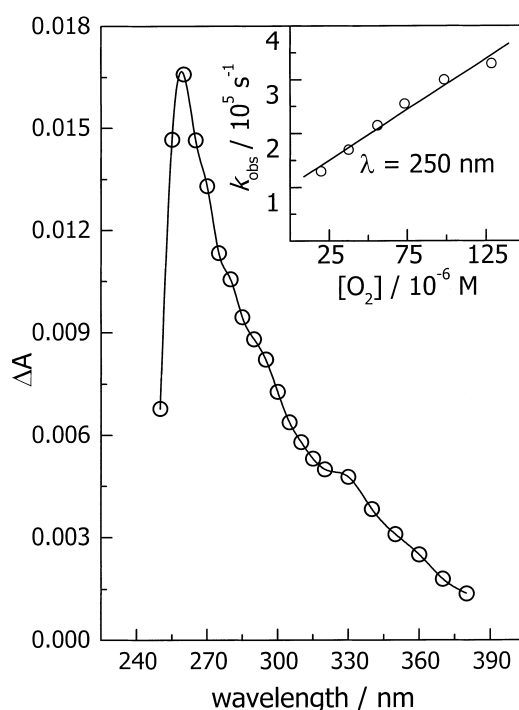
Fig. 7. Absorption spectrum of \text{CF}_2\text{BrO}_2^\bullet radical at 0.7 \mu\text{s} after the 500 ns electron pulse. [\text{CF}_2\text{Br}_2] = 1.55 \times 10^{-2} M; [\text{O}_2] = 2.7 \times 10^{-4} M; dose = 56 Gy. Inset: Dependence of observed rate constant of \text{CF}_2\text{Br}^\bullet radical decay on the concentration of oxygen.
