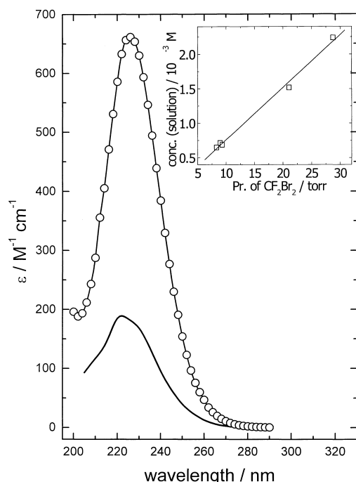
Fig. 3. Absorption spectra of CF 2 Br 2 in gas phase (○) and aqueous solution (—). Inset: Measurement of Henry's law constant ( K_h ).
