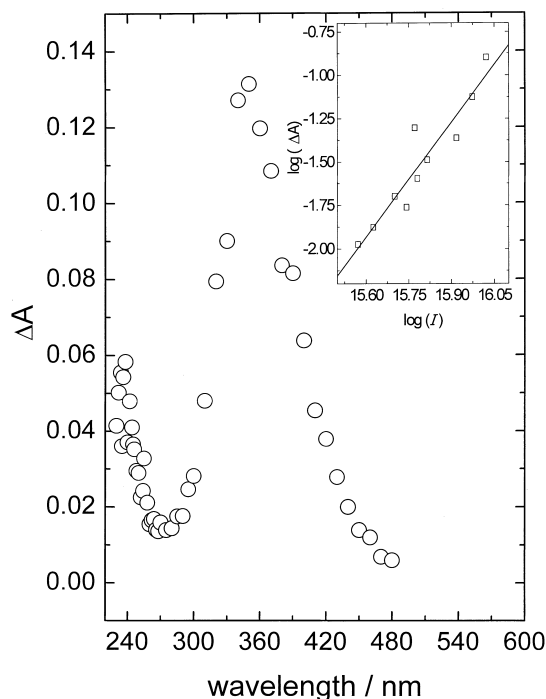
Fig. 4. Transient absorption spectrum, 3 \mu s after 248-nm laser flash. [\text{CF}_2\text{Br}_2] = 6.7 \times 10^{-3} M. Inset: Dependence of peak absorbance (350 nm) on laser intensity.
